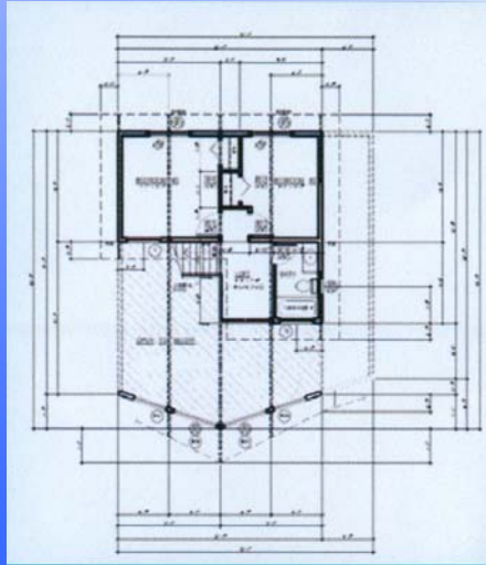
UPPER FLOOR 427.24 SQ. FT.
